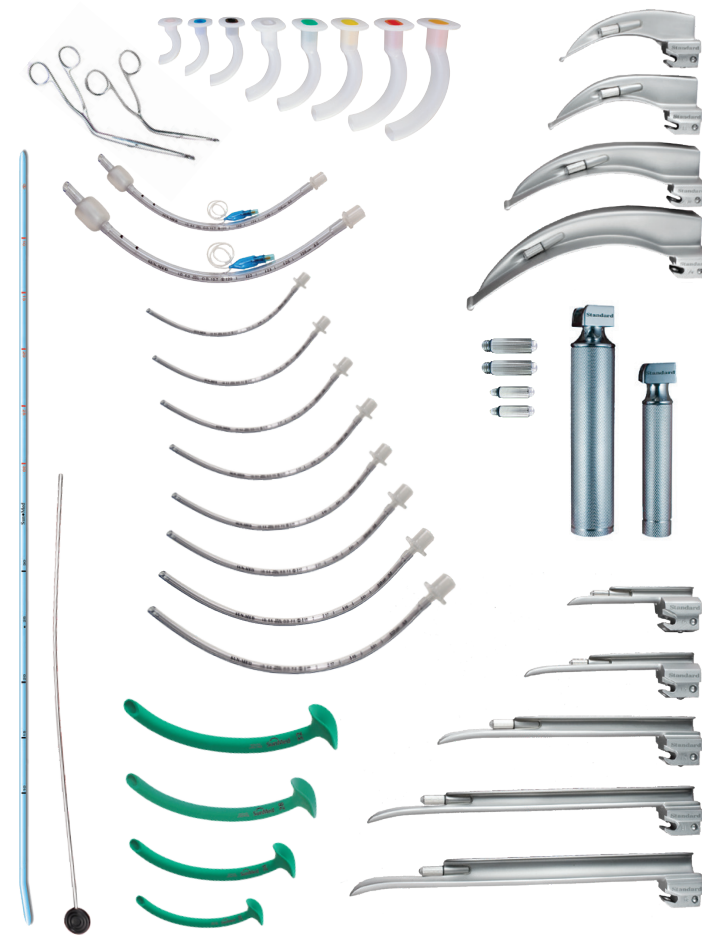
8-1050-85 Conventional Intubation Kit Batteries, lubricating jelly, and syringe not shown.
